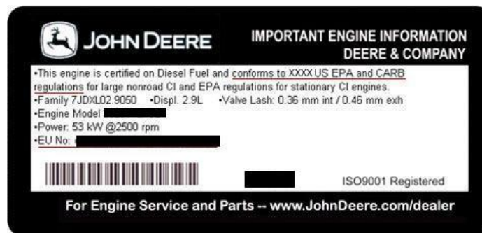
Figure 2-2 Example Emission Label for a Certified Engine
